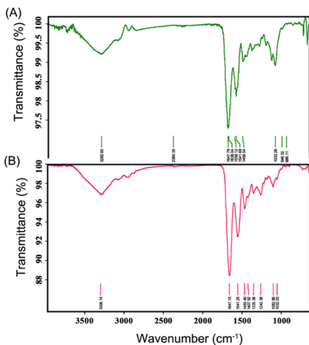
Figure 2. FTIR spectra of electrospun gelatin/hyaluronic acid fibres; (A) 93:7 and (B) 97:3.
