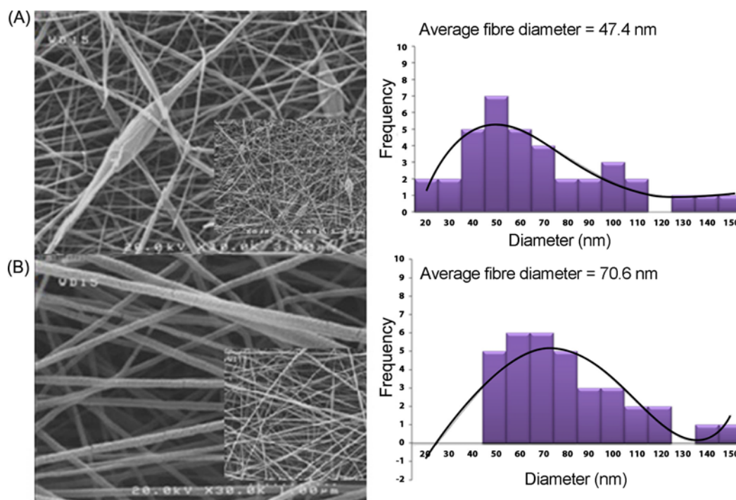
Figure 1. SEM micrographs (magnification=3000× and 30000×, scale bar=5 μm) and histogram distribution of fiber diameter of electrospun gelatin/hyaluronic acid fibres; (A) 93:7 and (B) 97:3.
